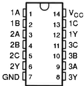
74HC10 Triple 3-input NAND
