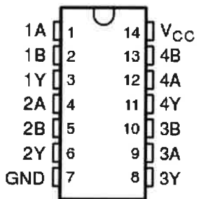
74HC86 Quad 2-input XOR
