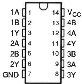
74HC00 Quad 2-input NAND
